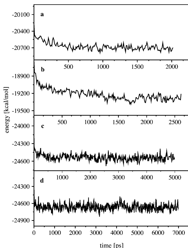
FIGURE 2 Total potential energy of our system (coarse grained over 10 ps) for the 4th, 8th, 12th, and 16th steps, (a–d) with respect to the simulation time.
