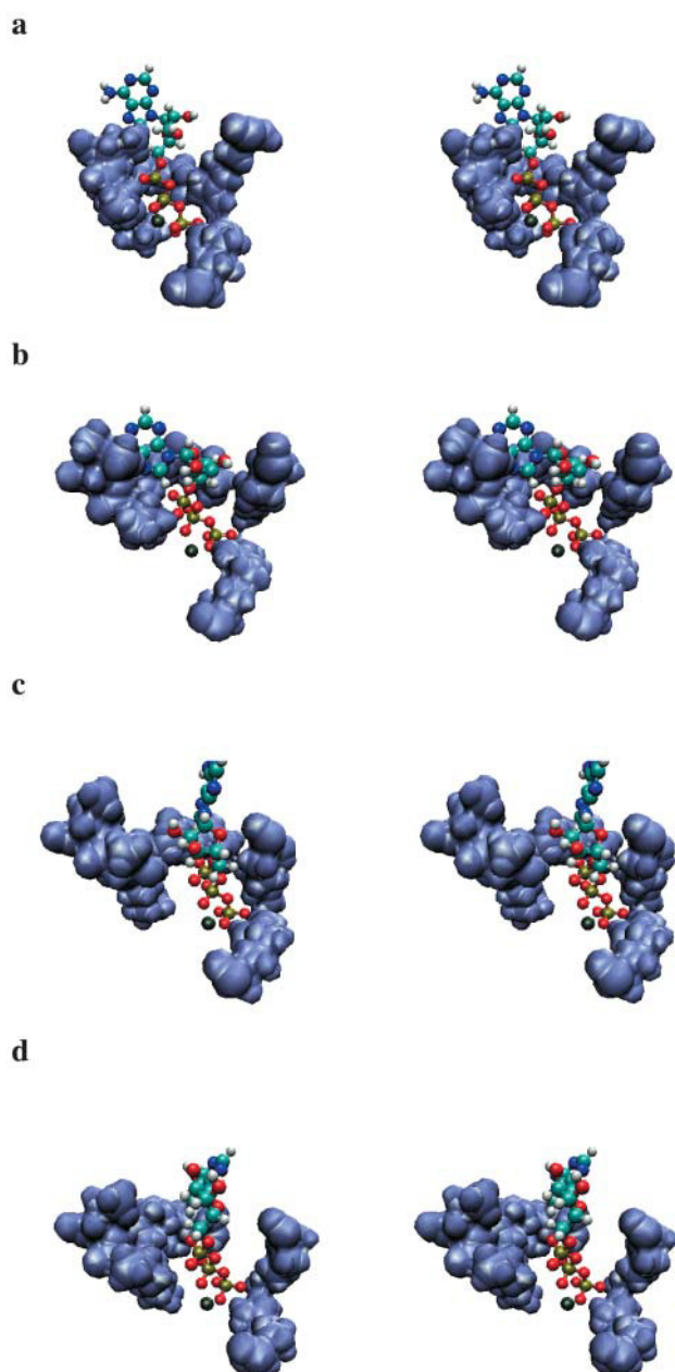
FIGURE 4 Stereo pictures of the hydrogen binding region and ATP. (a) Closed state, (b) 8th step, (c) 13th step, (d) open state. The orientation is the same as in Fig. 1 f. The pictures were created with VMD (Humphrey et al., 1996).
