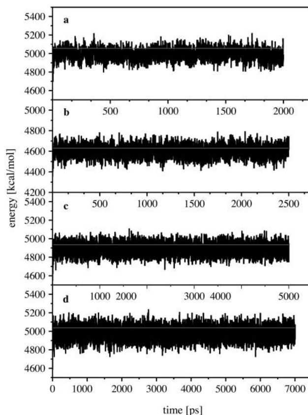
FIGURE 3 Total kinetic energy of our system for the 4th, 8th, 12th, and 16th steps, (a–d) with respect to the simulation time. The horizontal lines show the expected kinetic energy according to equipartition of the energy.
